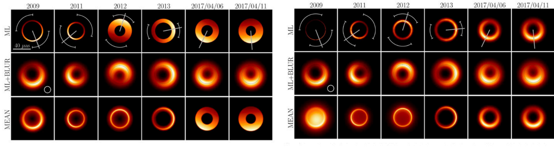
Figure 10. Images of M87* obtained by fitting two ring models to the EHT datasets 2009–17.
